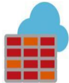
Firewall
