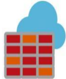
Firewall
